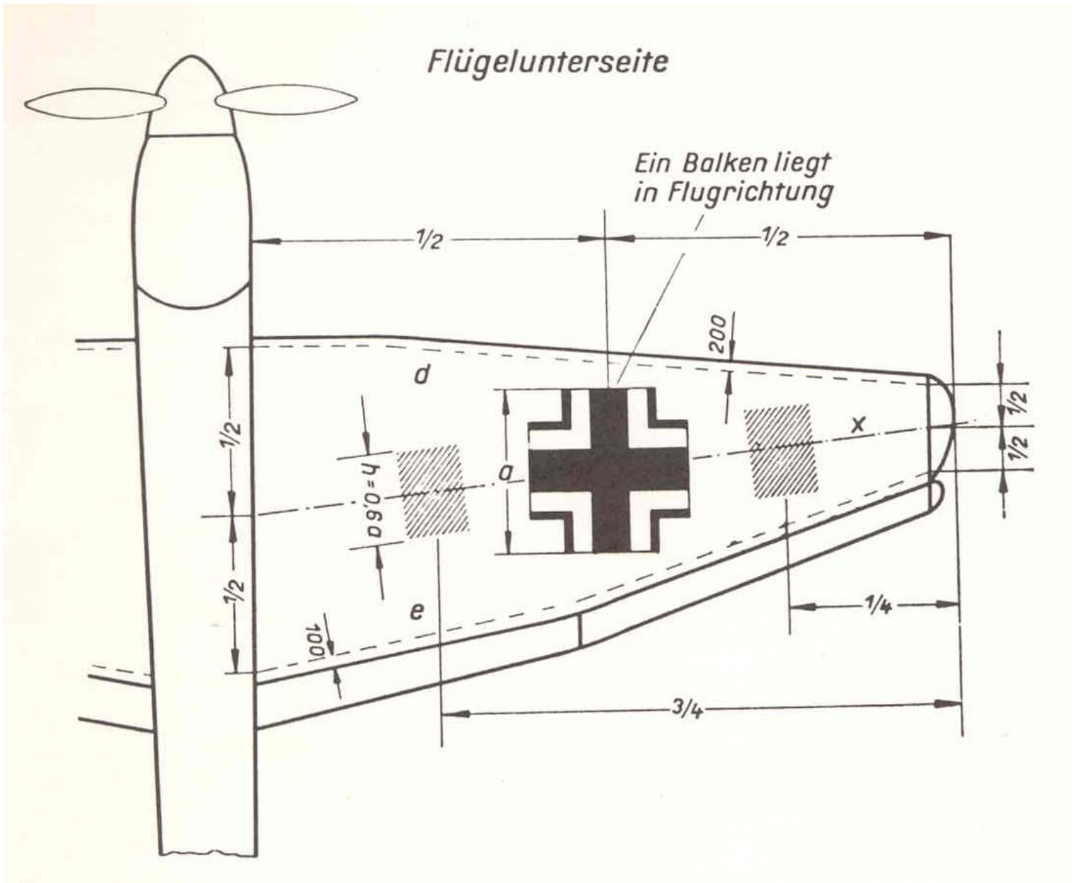
Location of markings & codes on wing lower surfaces for single-engine aircraft
